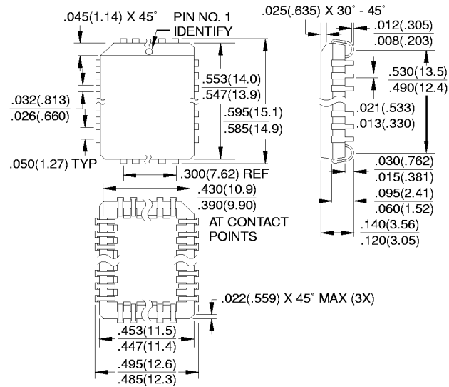
32J, 32-Lead, Plastic J-Leaded Chip Carrier (PLCC) Dimensions in Inches and (Millimeters) JEDEC STANDARD MS-016 AE
